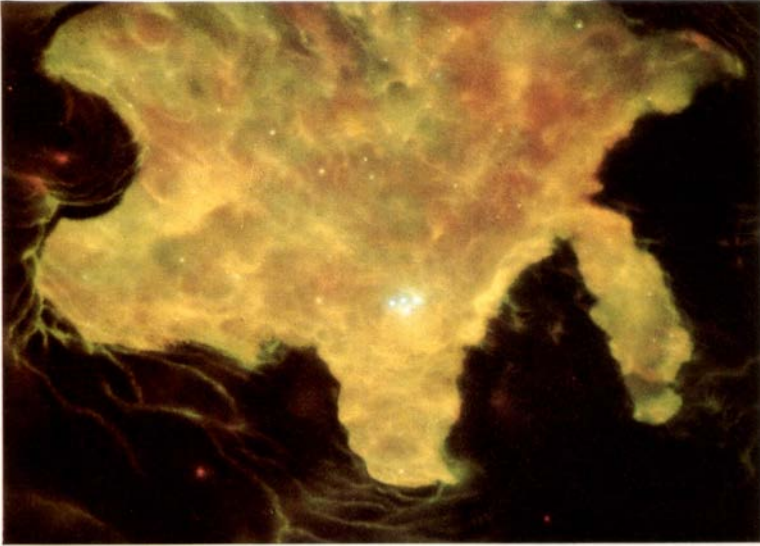
We emerge through the dark dust of the Orion Nebula to its hidden interior, brilliantly illuminated by hot young stars. Painting by John Allison.
