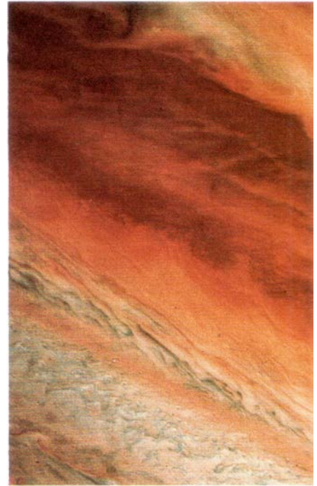
Voyager 2 image taken July 6, 1979, shows a region of the Jovian atmosphere from approximately 25°N to the equator. The north temperate "jet" of clouds is the rusty band running diagonally across top-mid frame. These clouds are moving at about 540 kilometers per hour. The bluish-white regions at bottom show breaks in the upper ammonia clouds. We are seeing approximately 60 kilometers down. Courtesy NASA.
