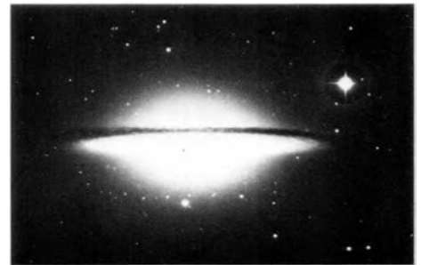
The Sombrero Galaxy, M104 (also called NGC 4594). The spiral arms, marked by lanes of dust, are tightly wound about its nucleus of stars. It is some 40 million light-years away, beyond the stars in the constellation Virgo, and may contain a trillion suns. Seen edge-on from some comparable distance, our spiral galaxy, the Milky Way, would resemble M104. Courtesy Hale Observatories.
