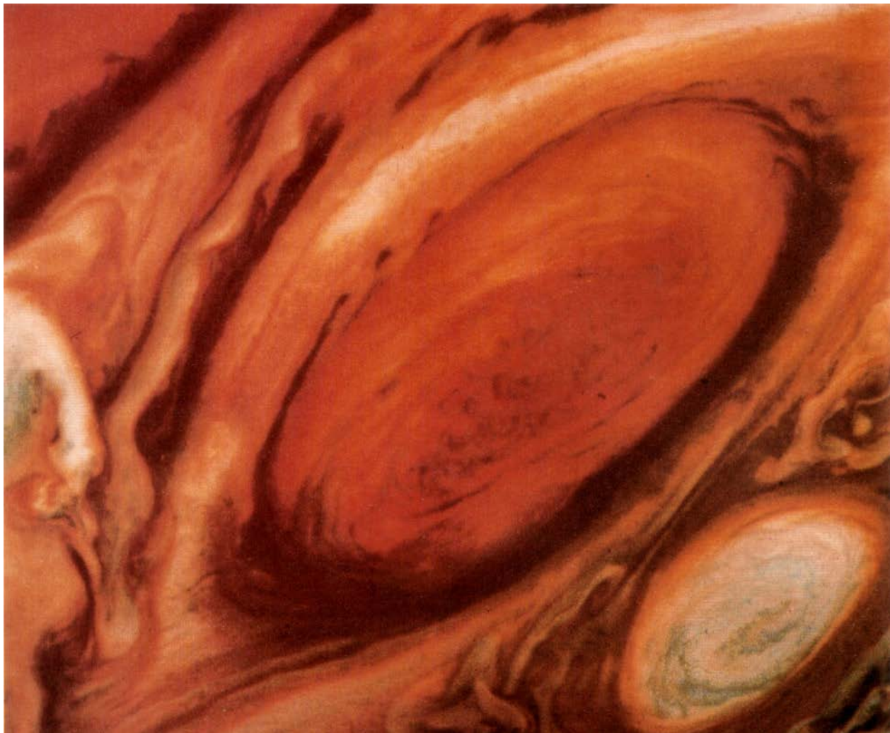
The Great Red Spot of Jupiter, a giant storm system 40,000 kilometers long and 11,000 kilometers wide rising above the adjacent clouds. It was first observed in 1664 by Robert Hooke and later confirmed by Christiaan Huygens. The material in the Red Spot rotates once every six Earth days; the white oval, lower right, rotates in the opposite sense. At top left are clouds overtaking the Red Spot from right to left. The reason the spot is red is unknown, as is the reason that there is only one Red Spot of this size. Voyager 2 image, courtesy NASA.
