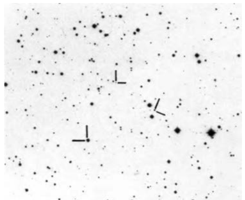
A deep sky survey in X-rays (top) within the constellation Eridanus, performed by the Einstein High-Energy Astrophysical Observatory in Earth orbit. The same region in ordinary visible light is shown at bottom, with three quasars indicated. Courtesy Ricardo Giacconi and NASA.
