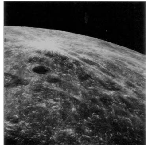
The rayed crater Bruno ( top ) on the Moon. Apollo Orbiter photo. Courtesy NASA.
