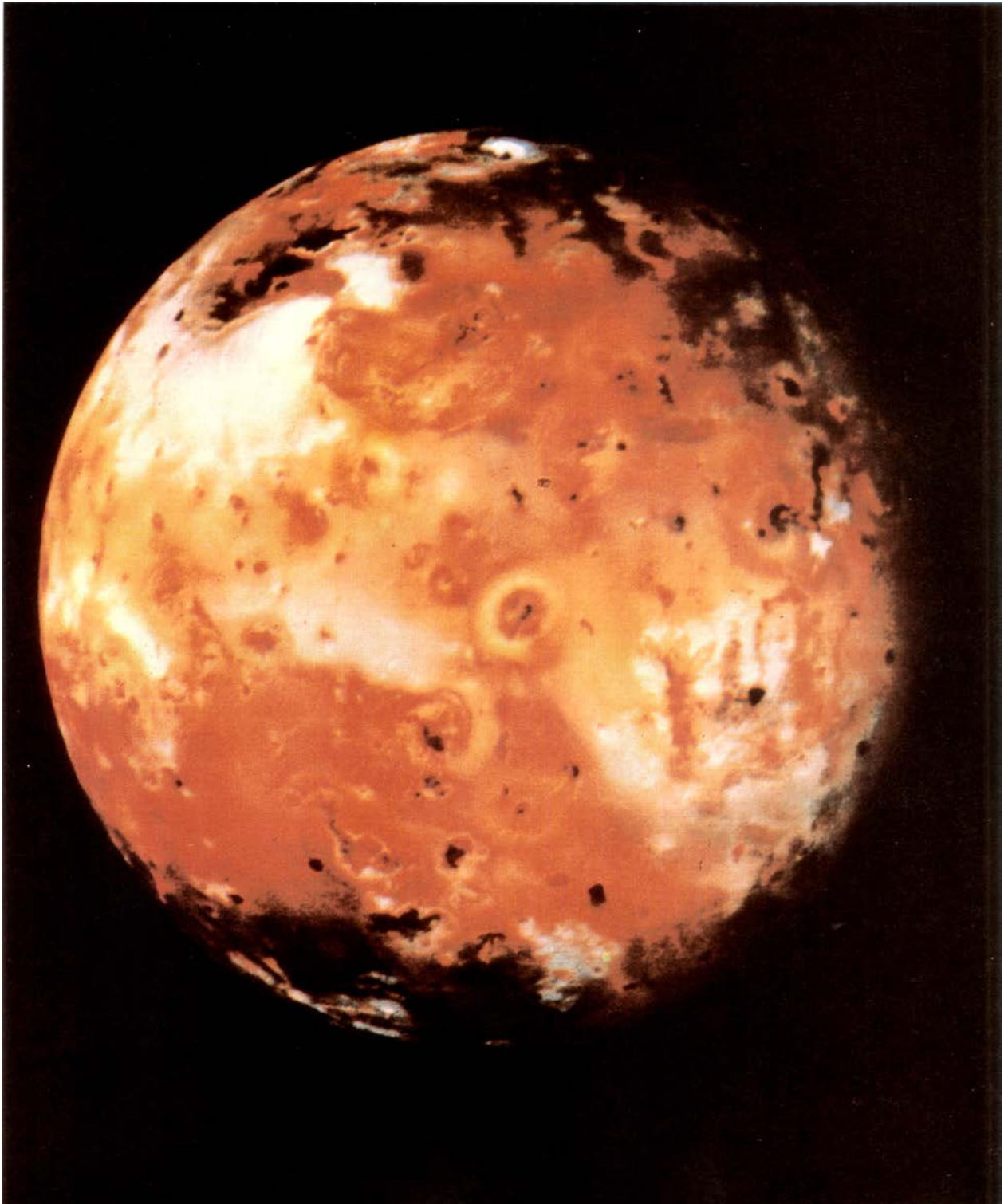
Voyager 1 image of the surface of Io. Each of the dark, roughly circular features is a recently active volcano. The volcano with a bright halo at the rough center of the disc was observed in eruption just fifteen hours before this image was acquired; it has since been named Prometheus. The black, red, orange and yellow colors are thought to be frozen sulfur, originally spewed from the volcanoes in a molten state, with the initial temperatures highest for black deposits and lowest for yellow. White deposits, including those around Prometheus, may be frozen sulfur dioxide. Io is 3,640 kilometers in diameter. Courtesy NASA.
