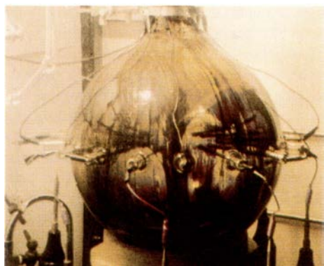
Synthesis of organic matter at the Laboratory for Planetary Studies, Cornell University. A transparent mixture of the gases methane, ammonia, hydrogen sulfide and water begins to be sparked in a glass flask ( top ). After a few hours of sparking, the interior of the flask is coated ( bottom ) with a rich variety of organic molecules relevant for the origin of life. Courtesy Bishun Khare.
