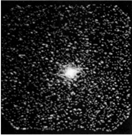
A photograph of the X-ray sky, showing the bright source Cygnus X-1 (center), a probable black hole. An image from High Energy Astrophysical Observatory 2, in Earth orbit. Courtesy Ricardo Giacconi and NASA.
