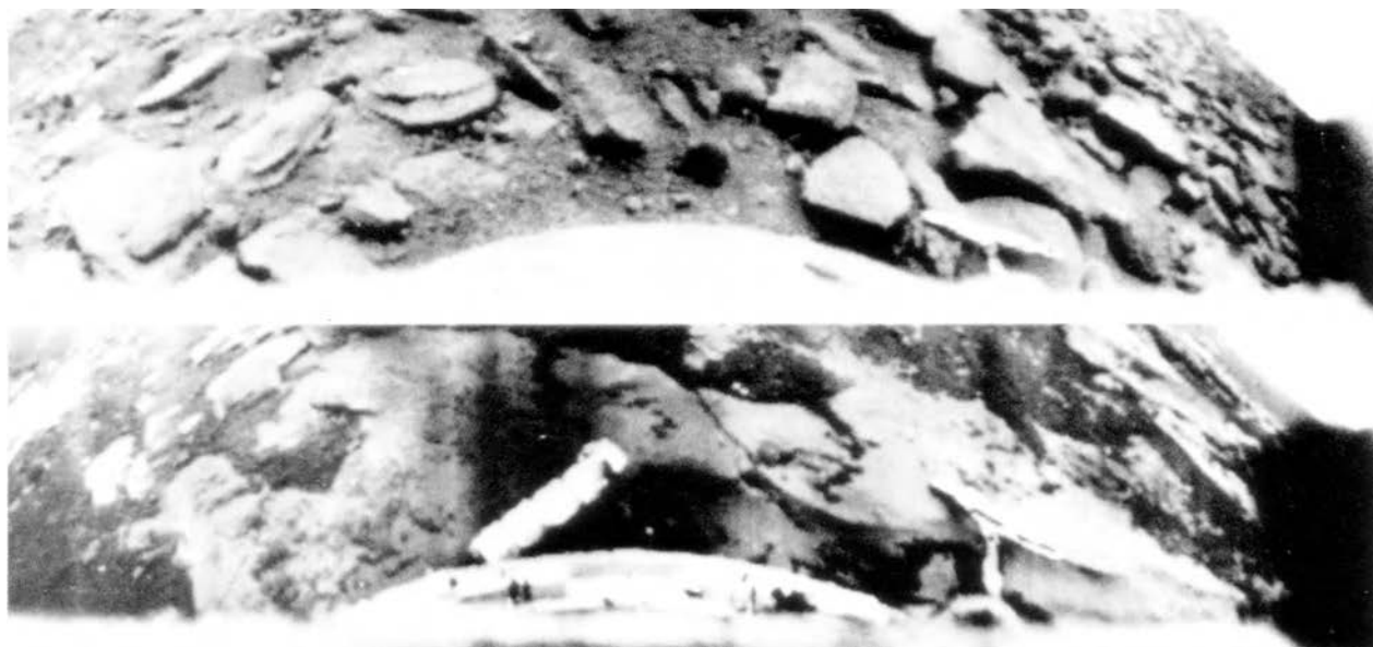
Venera 9 and 10 panoramic images of two different sites on the surface of the planet Venus. In both pictures the horizon is toward top right. Note the eroded form of the surface rocks. Courtesy Institute for Cosmic Research, Soviet Academy of Sciences, Moscow.
