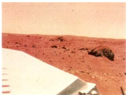
The sand-topped boulder known as “Big Joe” in Chryse. Had Viking 1 landed on it, the spacecraft would have crashed. Courtesy NASA.
