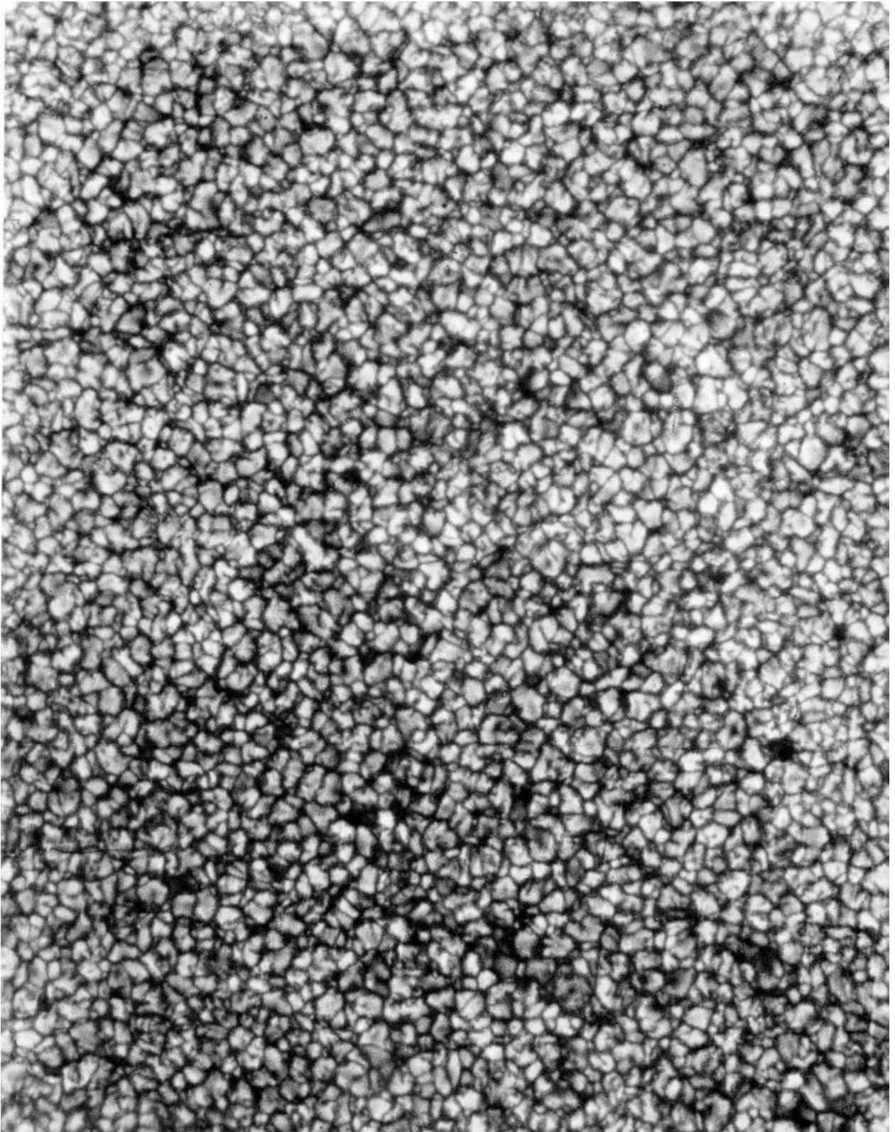
The turbulent surface of the Sun. Shown is the granulation, the solar provinces in which hot gas rises and sinks. Each turbulent cell is about 2,000 kilometers across, about the distance from Paris to Kiev. Photograph in ordinary yellow light from Pic du Midi Observatory, France.
