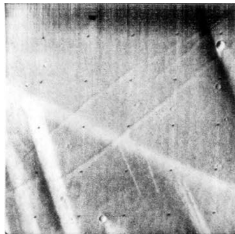
Unexplained linear markings on the Tharsis plateau. Mariner 9 photo, courtesy NASA.
