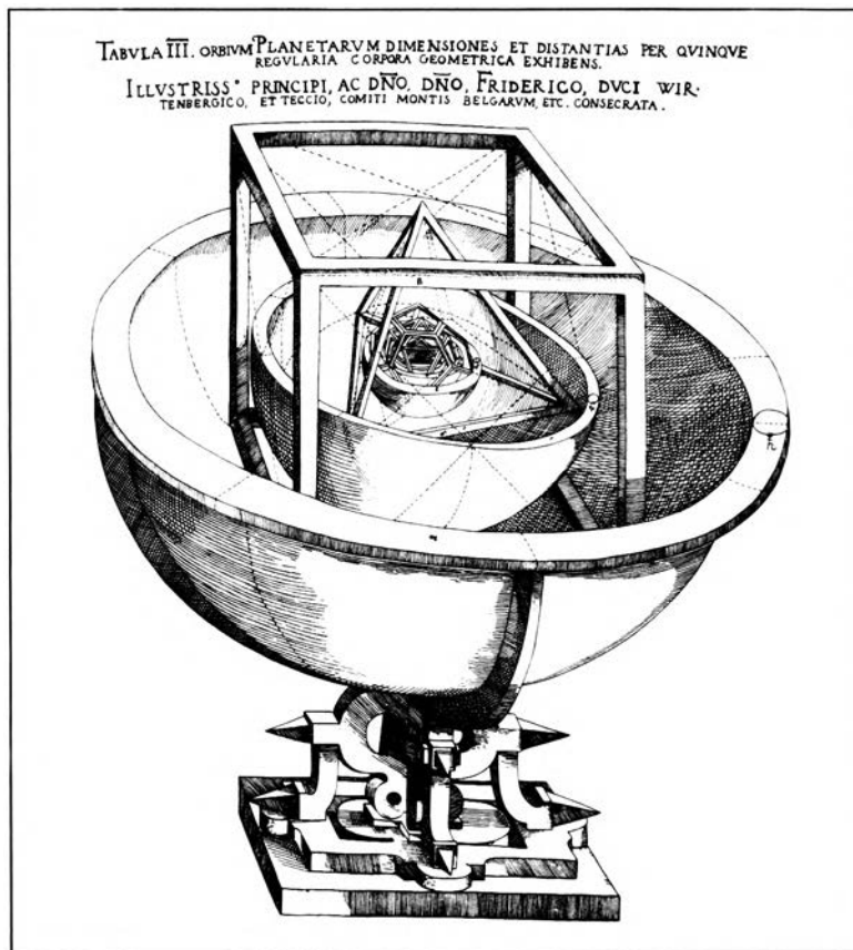
Kepler’s Cosmic Mystery, the spheres of the six planets nested in the five perfect solids of Pythagoras and Plato. The outermost perfect solid is the cube.
