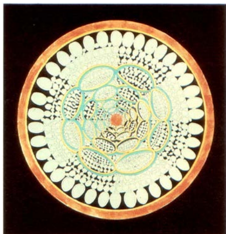
A schematic representation of an advanced technical civilization which rebuilds its solar system into a spherical shell of matter surrounding the local Sun, so the valuable starlight is not mainly lost to space. Painting by Jon Lomberg.
