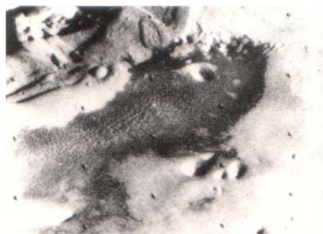
Portions of the great Mariner Valley, Vallis Marineris. Discovered in 1971-72 by Mariner 9, it is 5,000 kilometers long and roughly 100 kilometers wide. In model ( top ) are seen tributary valleys possibly caused by running water and wind-blown streaks associated with impact craters. Mariner 9 photos ( middle and bottom ) show avalanches that have collapsed walls and widened the valley and a giant dark sand dune field on the floor of Vallis Marineris. Courtesy NASA. Model by Don Davis.
