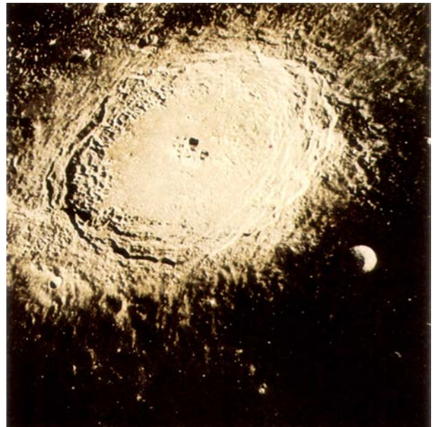
Dawn at Crater Copernicus, just north of the lunar equator. It is 100 kilometers in diameter. Its ray system is prominent when, unlike this photograph, it is illuminated directly face-on. Apollo Orbiter photo. Courtesy NASA.
