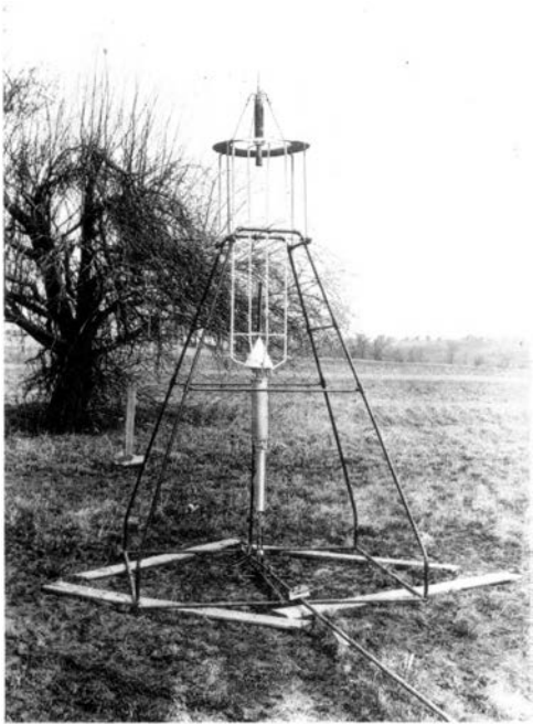
The first liquid-propellant rocket ever to fly. Launched by Robert Goddard on March 16, 1926, from the farm of his Aunt Effie in Auburn, Massachusetts, its flight lasted 2½ seconds. Courtesy Goddard Library, Clark University.
