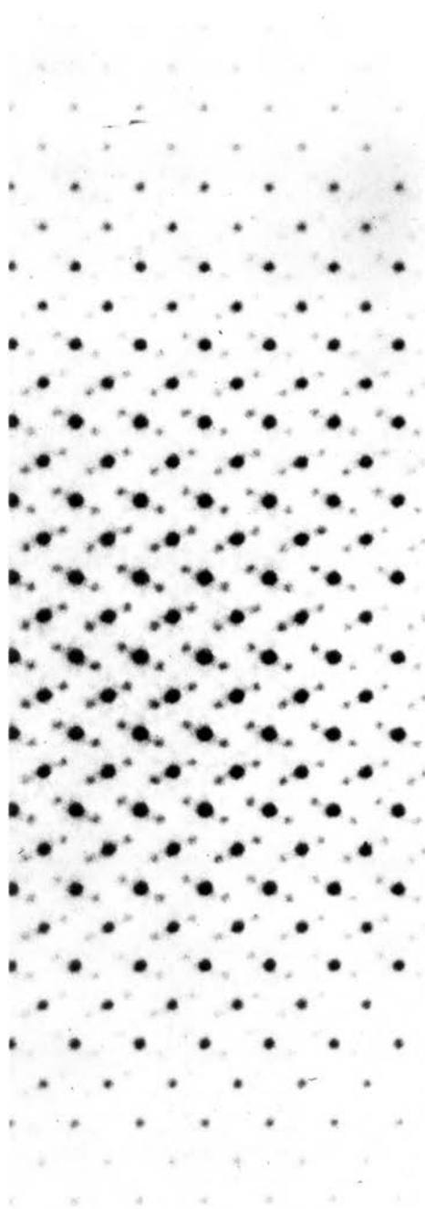
Atoms of the mineral marcasite, magnified 4-5 million times with a microscope employing both visible light and X-rays. Marcasite is a crystal in which the unit \text{FeS}_2 is repeated, Fe standing for iron and represented by the large spots, S standing for sulfur and represented by the pair of small spots flanking each iron atom. Courtesy Institute Professor Martin J. Buerger, Massachusetts Institute of Technology.
