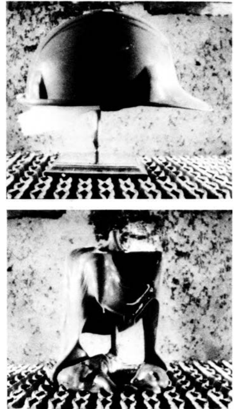
Plastic construction helmet before (top) and after (bottom) brief exposure to Venus surface temperatures. Photographed at Southwest Research Institute, San Antonio, Texas.
