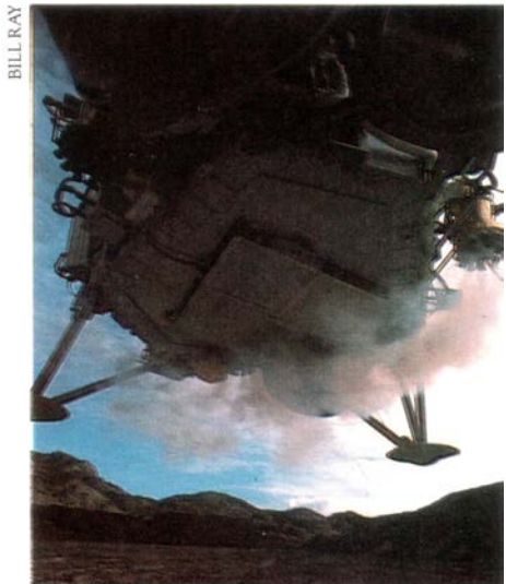
A simulated landing, in Death Valley, California, of Viking on Mars. The terminal stages of descent are braked by the firing of retrorockets.
