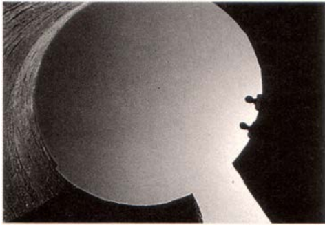
Looking up from the bottom of the well in ancient Syene, near present-day Abu Simbel, in Egypt, which according to local tradition is the origin of Eratosthenes' study of the circumference of the Earth.
