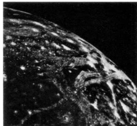
Ganymede, the largest moon of Jupiter. The smallest features visible in this Voyager 1 image are about three kilometers across. Numerous impact craters are evident, many with bright rays. The gently swerving and intersecting bands are composed of parallel grooves of uncertain origin. Courtesy NASA.
