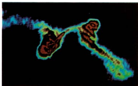
Radio image of elliptical galaxy NGC 3266. Imaged in false color by the Very Large Array.
