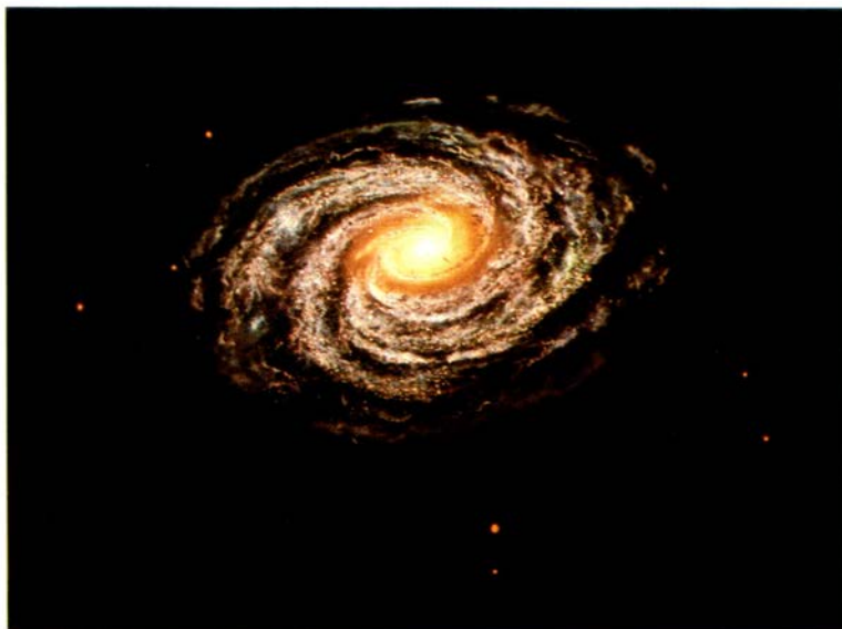
A typical spiral galaxy. Painting by Jon Lomberg.
