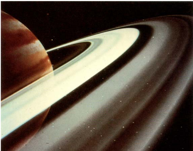
Pioneer 11 image of Saturn and its rings obtained from a range of 2.5 million kilometers on August 29, 1979, after a voyage of more than five years. Courtesy NASA.
