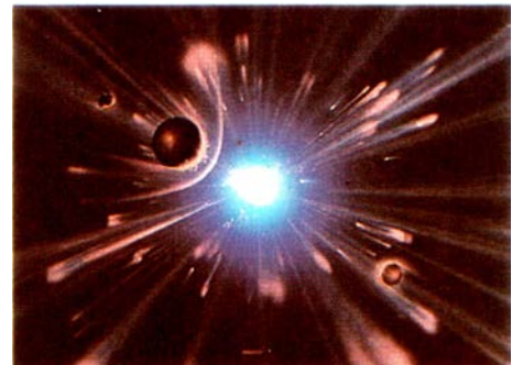
The death of a solar system. Schematic views of the loss of planetary atmospheres and the vaporization of worlds when the local sun becomes a supernova. The shock waves we see propagate beyond the local system, compress the interstellar gas and dust, and lead to the formation of new planetary systems. Paintings by Adolf Schaller, Rick Sternbach and John Allison.
