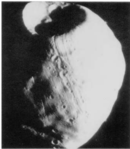
Phobos, the innermost moon of Mars. Crater Stickney is shown at top. If the impacting object that produced this crater had been a little larger, Phobos might have been disintegrated. Viking 1 Orbiter photo. Courtesy NASA.
