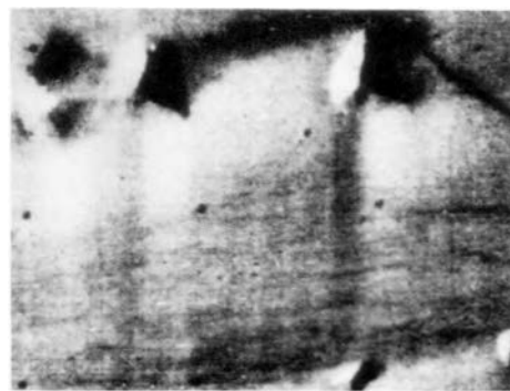
The pyramids of Elysium. Mariner 9 photo. Courtesy NASA.
