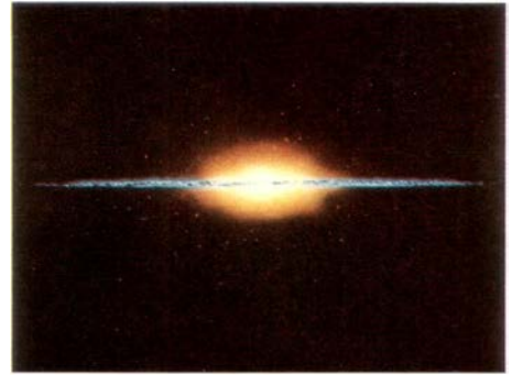
Schematic representation of the Milky Way viewed edge-on, surrounded by a swarm of globular star clusters, each containing between one hundred thousand and ten million stars. On this scale the Sun and Earth lie close to the outer edge of the spiral arms, jutting out from the galactic core. Painting by Jon Lomberg.
