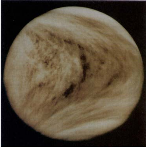
Full-disk view of Venus in ultraviolet light, printed in the hues of the visible spectrum. The patterns are due to clouds, rotating right to left, high in the Venus atmosphere. Pioneer Venus Orbiter photo. Courtesy NASA.
