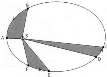
Kepler's second law: A planet sweeps out equal areas in equal times. It takes as long to travel from B to A as from F to E as from D to C; and the shaded areas BSA, FSE and DSC are all equal.
