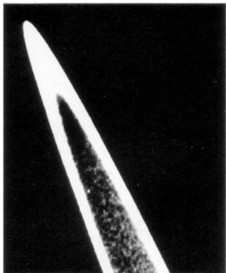
The rings of Jupiter, discovered by Voyager 1 and here photographed by Voyager 2. Jupiter is out of frame at lower right. Composed of small particles, it seems to extend all the way down to the Jovian cloudtops, suggesting a steady state between production, perhaps from material escaping from Io, and destruction by entry into the clouds of Jupiter. It is much smaller and dimmer than the rings of Saturn, accounting for the fact that it was never reliably discovered from Earth before Voyager. Courtesy NASA.
