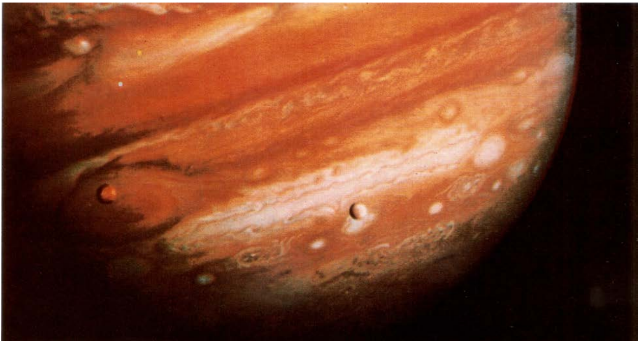
Voyager 1 far encounter image ( top ) of Jupiter from a range of 28 million kilometers. Bottom : Voyager approaches Jupiter with the moons Io and Callisto in foreground. Courtesy NASA.
