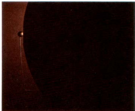
As the star is totally occulted, the planet emerges from the glare. Repeated such observations could determine the position, motion and perhaps other properties of the previously undiscovered planet.
