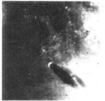
Dark, possibly volcanic material blown by winds out of a crater in Mesogaea on Mars. Mariner 9 photo. Courtesy NASA.
