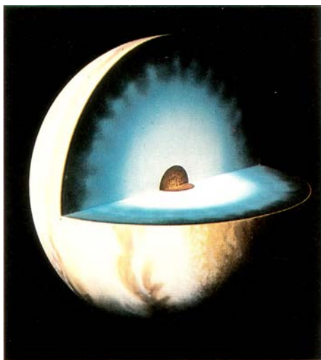
Cutaway model of the interior of Jupiter. On this scale, the visible clouds are thinner than the paint on the exterior of the model's surface. At the core is a sphere of rock and metal a little like the Earth, surrounding which is a great ocean of liquid metallic hydrogen.
