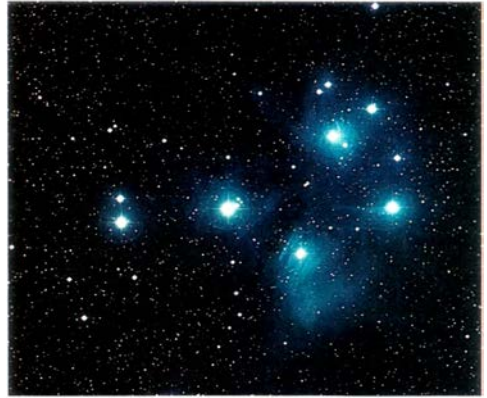
The Pleiades in the constellation Taurus, first examined through the telescope by Galileo. The spectra of the blue nebosity is the same as that of the nearby stars, showing the nebosity to be dust, reflecting the light of the newly-formed stars. About 400 light-years away, the brighter stars were named by the ancient Greeks after the daughters of Atlas, the Titan who held the heavens up. Courtesy Hale Observatories.
