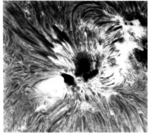
Close-up of a sunspot group in red hydrogen light. Sunspots are comparatively cooler regions with strong magnetic fields. The adjacent dark “spicules” are ordered by local magnetism, somewhat as iron filings are by a bar magnet. The adjacent bright “plages” are associated with the appearance of the great storms called solar flares. Courtesy Big Bear Solar Observatory.
