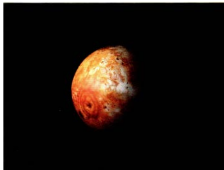
Io, the innermost large moon of Jupiter. Model by Don Davis.
