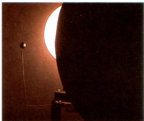
As the starlight is artificially eclipsed by a foreground occulting disk (or the lunar surface), the planet, shining by reflected light, becomes more easily seen.
