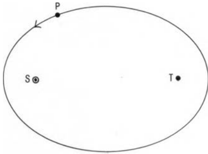
Kepler's first law: A planet (P) moves in an ellipse with the Sun (S) at one of the two foci.
