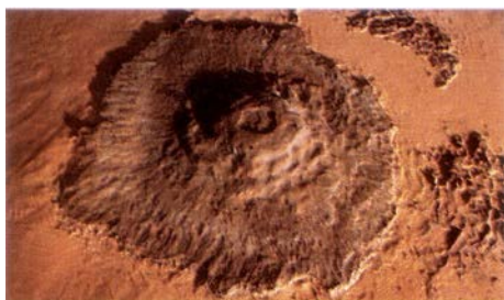
Top: Viking Orbiter color mosaic of three of the four great volcanoes in Tharsis on Mars and the western provinces of Vallis Marineris. Mariner 9 image ( middle ) and model ( bottom ) of Olympus Mons, Mount Olympus, the largest volcanic construct definitively identified in the solar system to date. Its area is about the size of Arizona and it is almost three times the height of Mount Everest. It was constructed at a time of great geological activity on Mars about a billion years ago. Courtesy NASA. Model by Don Davis.
