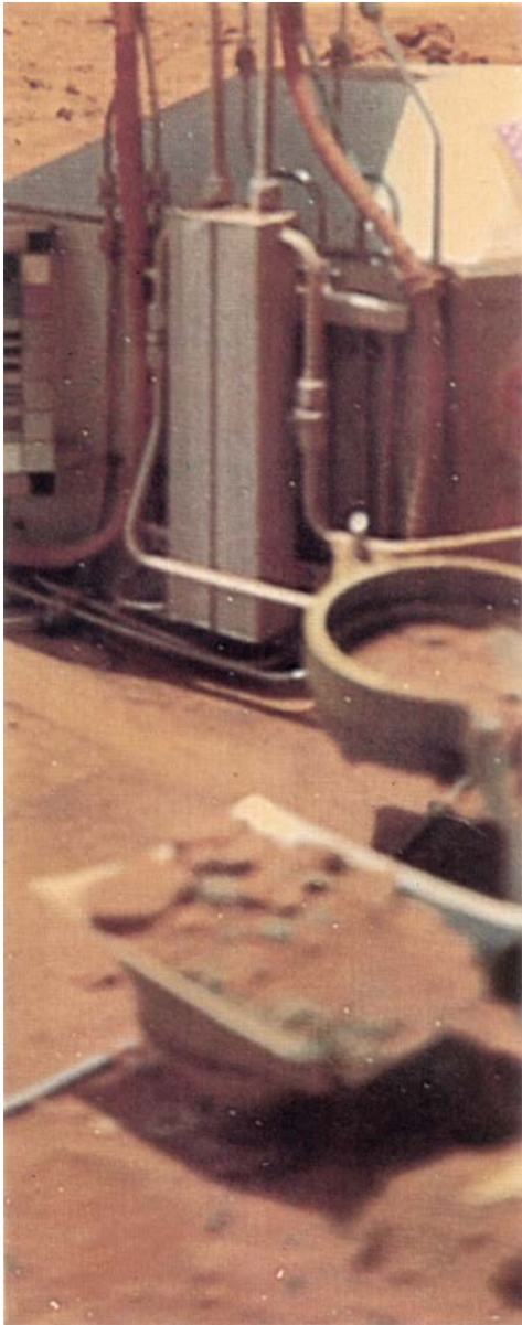
Sand and small stones deposited by the Viking 2 surface sampler in the inlet to the X-ray fluorescence spectrometer ( out of focus, bottom center ), a device to determine the inorganic chemistry of Martian soil. Inlets nearby lead to the organic chemistry and microbiology experiments. Courtesy NASA.
