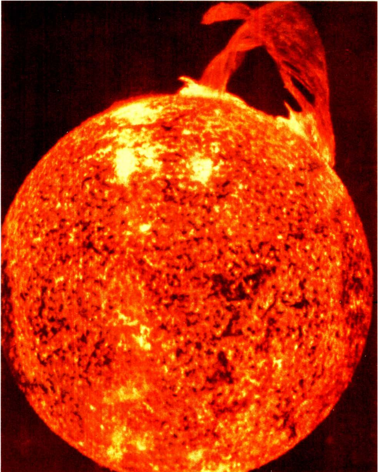
The nearest star: the Sun seen in the light of ionized helium in the far ultraviolet. The solar prominence surging at top right extends momentarily some 300,000 kilometers into space until it falls back on the glowing gas that is the Sun's visible surface. The smallest patches of hot gas visible on this image of the solar surface are about the size of the Earth. Skylab 4 photo, courtesy NASA.
