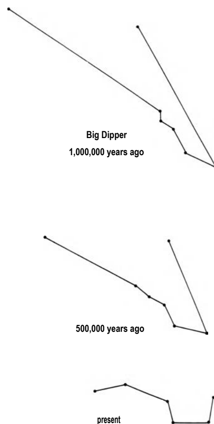
Computer-generated images of the Big Dipper as it would have been seen on Earth one million years ago and half a million years ago. Its present appearance is shown at bottom.
