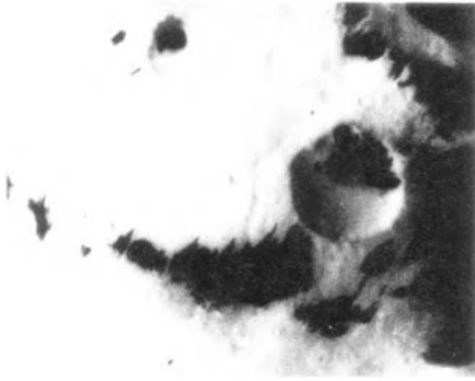
Dark variable markings in and near craters in Memnonia on Mars. Drifting bright sand and dust covers and uncovers underlying dark material. Windblown fine particles also cover over and erode craters and other geological forms. Mariner 9 photo. Courtesy NASA.
