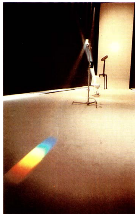
A spectrum produced when a bright light passes through a slit and then through a glass prism. If a gas that strongly absorbed visible light were in the light path, the rainbow pattern would be interrupted by a set of dark lines characteristic of the gas.
