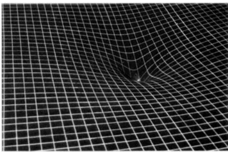
Schematic representation of the distortion of flat space by a massive object, useful in thinking about gravitation and black holes.
