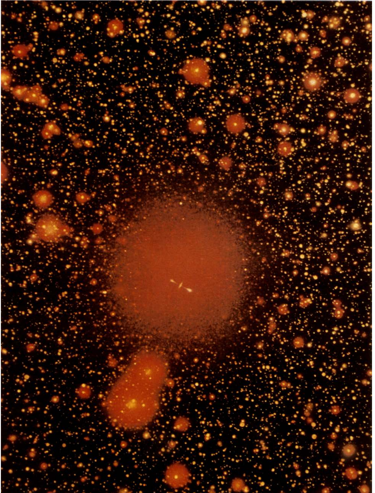
Quasar inside a giant elliptical galaxy, dominating a rich cluster of galaxies. Painting by Adolf Schaller.
