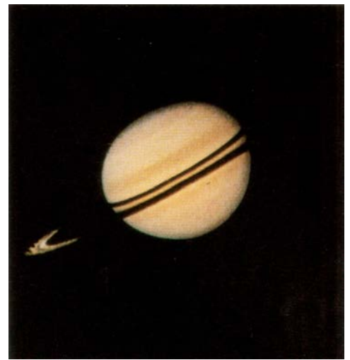
Pioneer 11 image of Saturn and its rings obtained from a range of 2.5 million kilometers on August 29, 1979, after a voyage of more than five years. Courtesy NASA.
