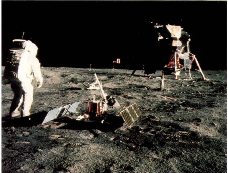
Apollo 16 astronaut sets up laser retroreflector experiment on the Moon. Courtesy NASA.
