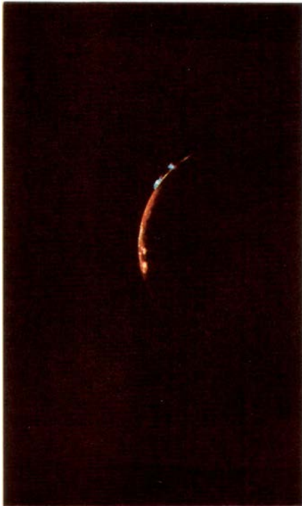
Two erupting volcanoes at the limb or edge of crescent Io. They had apparently been erupting continuously for four months. The lower plume is from the Maui Patera volcano. Voyager 2 image. Courtesy NASA.
