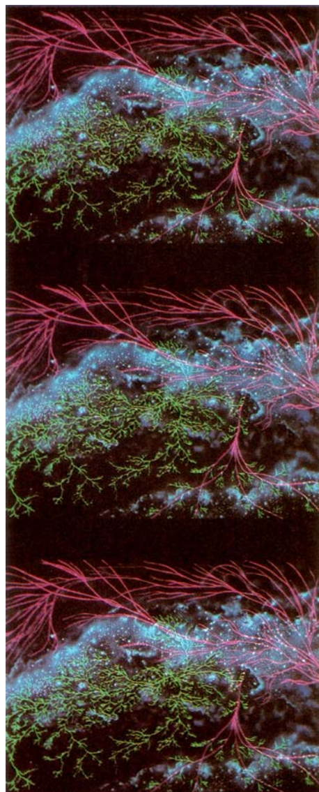
An interstellar colonial civilization, diffusing from star system to star system in comparatively short hops ( green ) encounters another such civilization ( red ), capable of longer journeys. Animation by Dov Jacobson.
