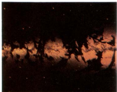
Dark cloud of interstellar dust. Such cloud complexes are filled with simple organic gases; the individual dust grains themselves may be composed in part of organic molecules. Painting by Adolf Schaller.
