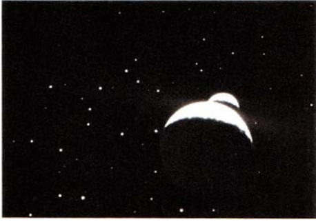
Pluto, covered with methane frost, and its giant moon Charon. Usually the outermost planet, Pluto's orbit has recently carried it interior to the orbit of Neptune. Painting by John Allison.
