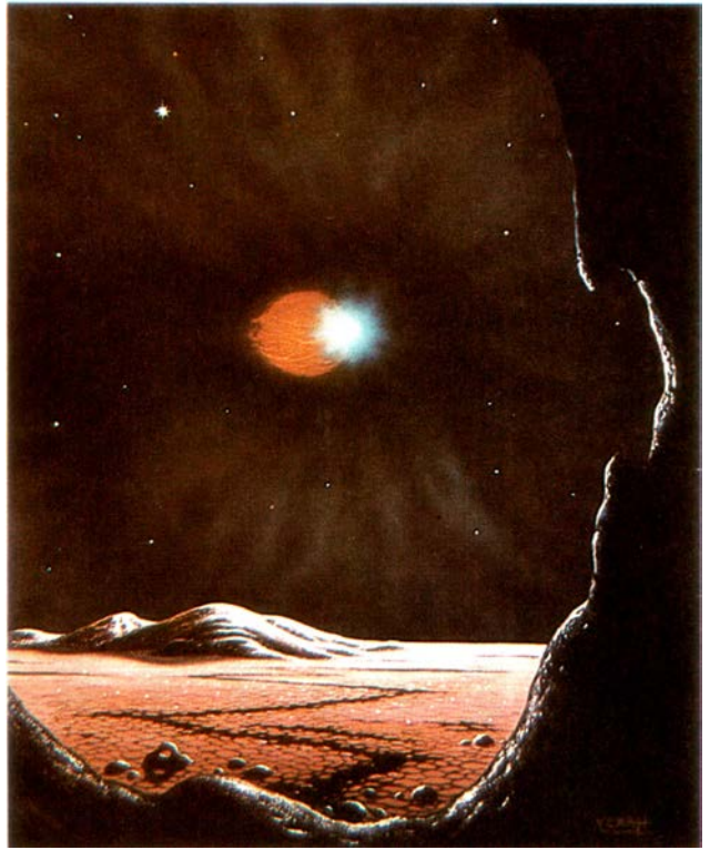
A contact binary, a red giant and a blue dwarf, the latter undergoing a nova explosion. The event has withered the planetary landscape. Painting by David Hardy. © David A. Hardy, from Challenge of the Stars (Rand McNally).
