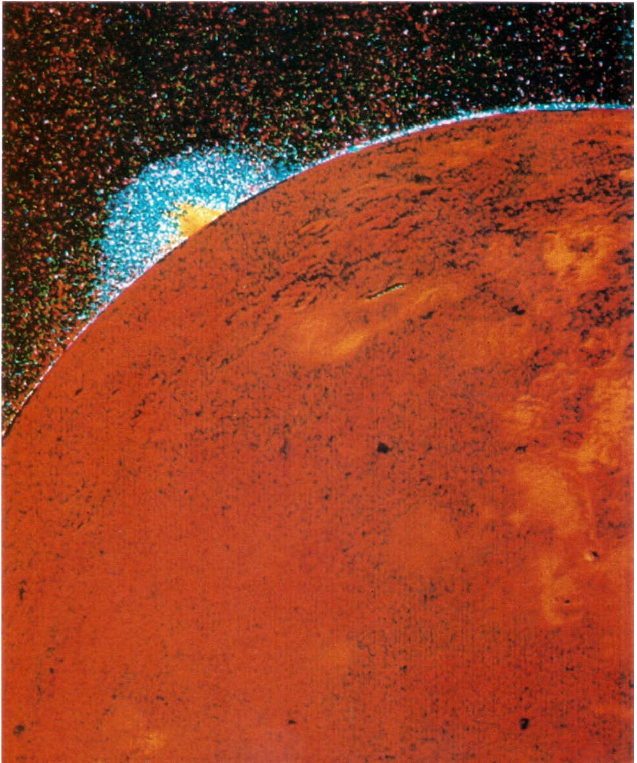
The volcanic plume of the Loki Patera volcano on Io. Ultraviolet light is here transcribed as blue. Surrounding the plume seen in visible light is a vast cloud, bright in reflected ultraviolet sunlight and composed of very small particles. The effect is similar to the blue cast of the light reflected by fine smoke particles. The top of the ultraviolet cloud is more than 200 kilometers above the surface of Io and may eject extremely small particles and atoms directly into space. The ejected matter would still be in orbit about Jupiter, as Io is, and supply the great tube of atoms which surrounds Jupiter at Io's distance. Voyager 1 image. Courtesy NASA.
