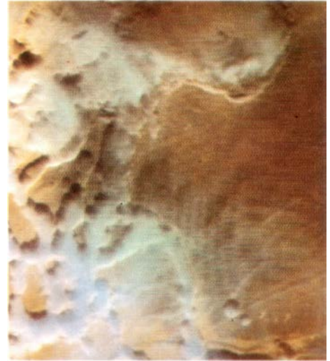
Morning haze and frost in the heavily eroded terrain of Noctis Labyrinthus, the Labyrinth of Night. Viking Orbiter photo, courtesy NASA.
