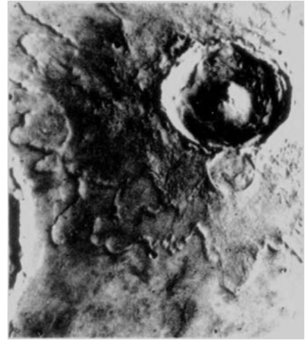
Crater Yuty at 22°N, 34°W on Mars. Surrounding it are several layers of surface material ejected in the impact that produced the crater. The splash pattern suggests that the excavated material flowed outward on some lubricant, probably subsurface ice melted by the impact. A small earlier crater just below Yuty has not been buried by the ejecta, indicating that the ejecta layer is thin. Mariner 9 photo. Courtesy NASA.
