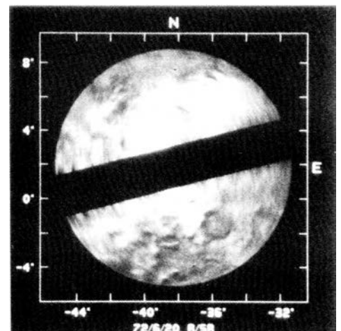
Close-up of an equatorial region on Venus as seen by radar astronomy from Earth. The diagonal bar is a region from which no useful data were returned. Several craters are seen, the largest almost 200 kilometers across. Craters on Venus are very shallow compared with crater of similar diameters on other worlds, hinting at some special erosion mechanism. Goldstone Tracking Station, Jet Propulsion Laboratory.
