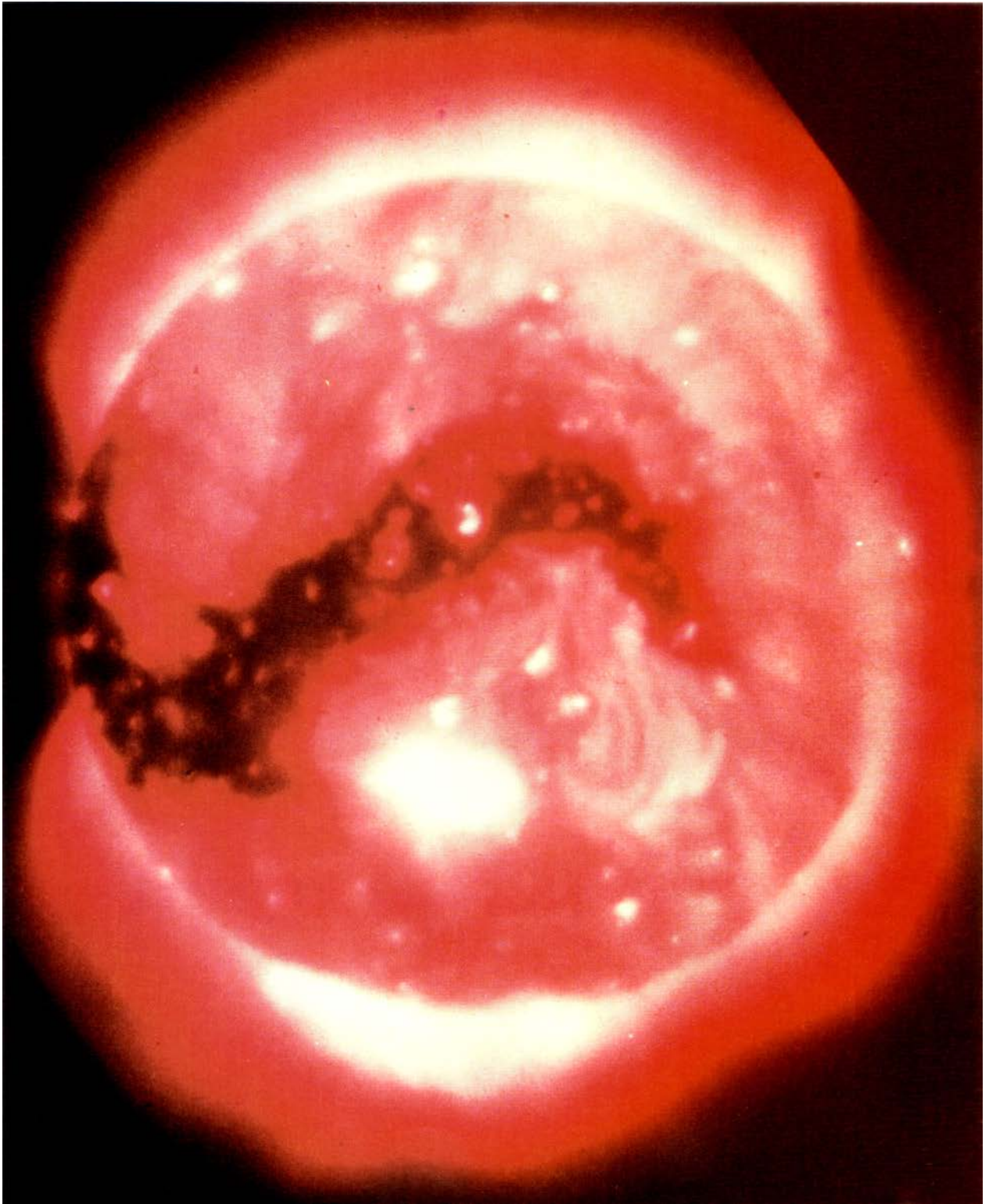
A hole in the corona of the Sun. Surrounding the solar photosphere is the thin outer atmosphere of the Sun, at a temperature of a million degrees, which changes its shape with the 11.2-year solar cycle. The corona is seen here in soft X-rays as a red halo about the Sun. The coronal hole is boot-shaped at center. Through such holes stream the protons and electrons of the solar wind, on their way past the planets to interstellar space. Skylab photo, courtesy NASA.
