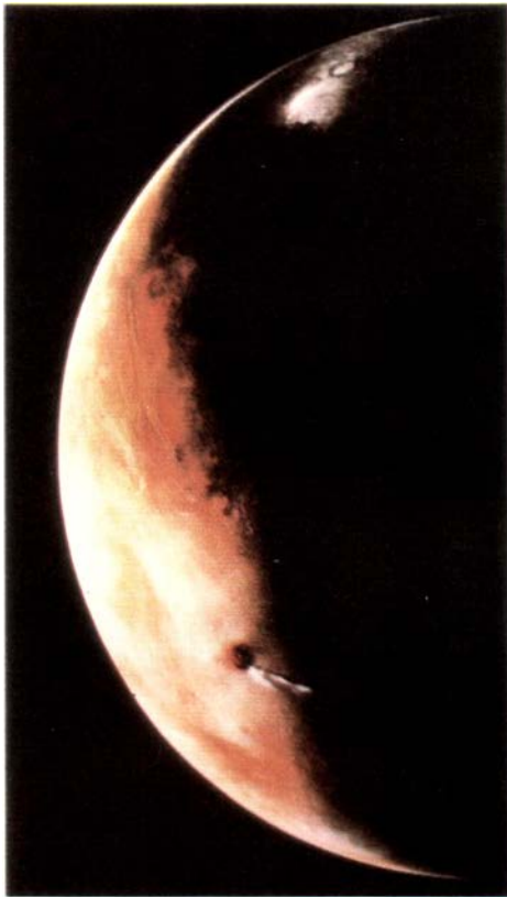
Viking far-encounter photograph of crescent Mars, showing crater in North Polar Cap, and orogenic clouds in the lee of the great Martian volcano, Olympus Mons. Courtesy NASA.
