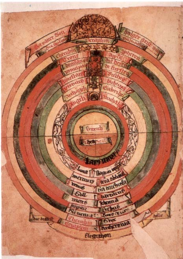
The geocentric pre-Copernican Universe in Christian Europe. At center, Earth is divided into Heaven (tan) and Hell (brown). The elements water (green), air (blue) and fire (red) surround the Earth. Moving outward, concentrically, are the spheres containing the seven planets, the Moon and the Sun, as well as the "Twelve Orders of the Blessed Spirits," the Cherubim and the Seraphim. German manuscript, c. 1450.
