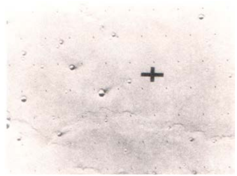
The bland terrain on Chryse Planitia on which Viking 1 landed. Touchdown occurred within a few kilometers of the target area, marked by the cross, after an interplanetary voyage of some hundred million kilometers. Courtesy NASA.
