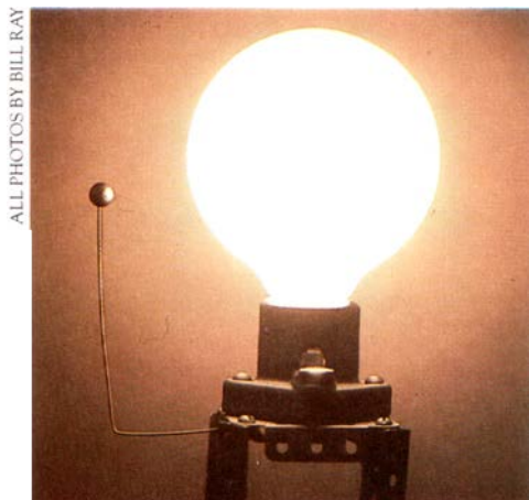
An electric light bulb, representing a distant star, and a small sphere representing a non-self-luminous planetary companion. Stars are so bright that their planets would ordinarily be totally lost in their glare.
