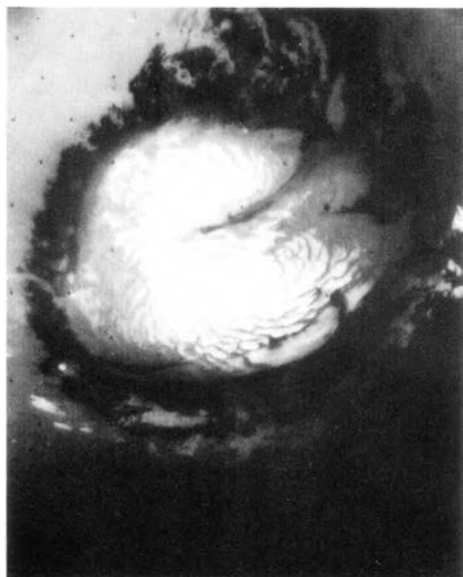
The North Polar Cap of Mars, surrounded by dark sand dune fields. This cap is made primarily of water ice; the South Polar Cap, mainly of frozen carbon dioxide. To darken the caps it would be cheaper to move the circumjacent sand than to carry material from Earth. But the winds would still scour the caps. Mariner 9 photo. Courtesy NASA.
