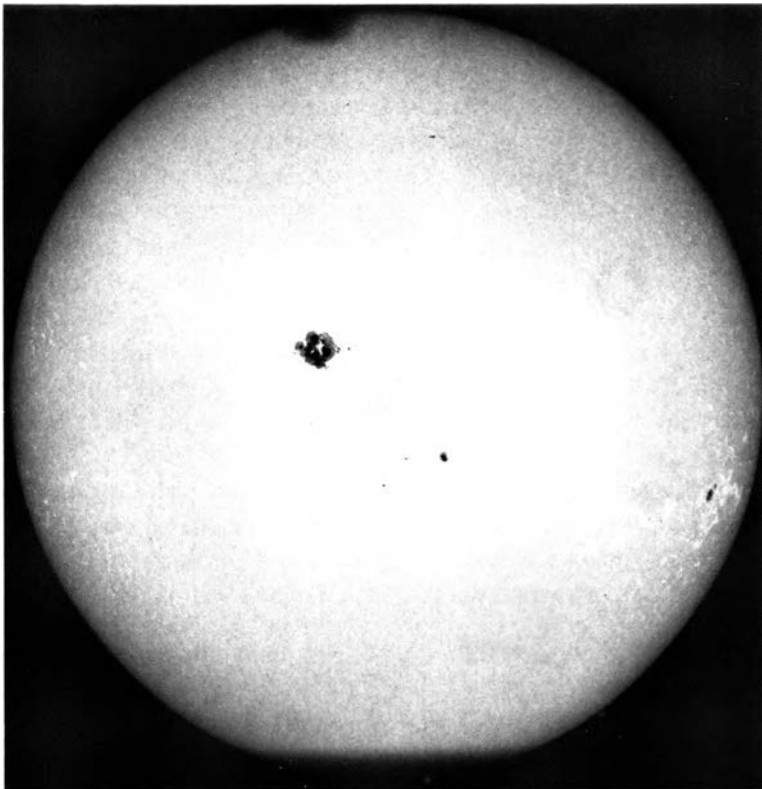
The photosphere of the Sun, the region in the solar atmosphere from which ordinary visible light is radiated to space. This photograph was taken near a maximum in sunspot activity, which recurs every 11.2 years. At such times there may be 100 separate sunspots visible. They are darker than their surroundings because they are about 2000°C cooler. Sunspots were first discovered by Galileo, although under favorable conditions—at sunset, for example—they can be seen with the naked eye. Courtesy Gary Chapman, San Fernando Observatory, California State University, Northridge.
