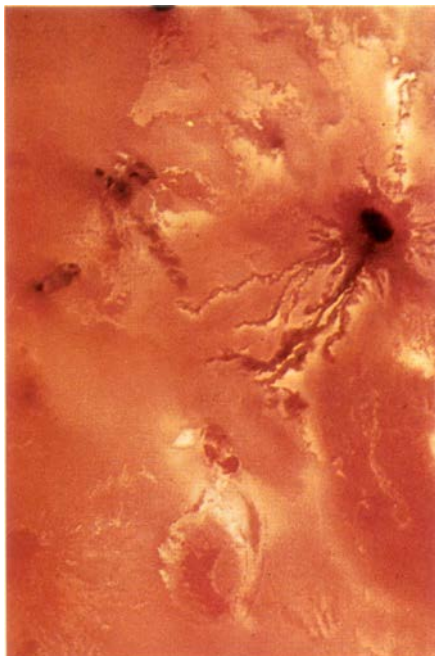
Recent flows of molten sulfur from the Ra Patera volcano on Io. We are viewing almost directly down the volcanic caldera. Voyager 1 image. Courtesy NASA.
