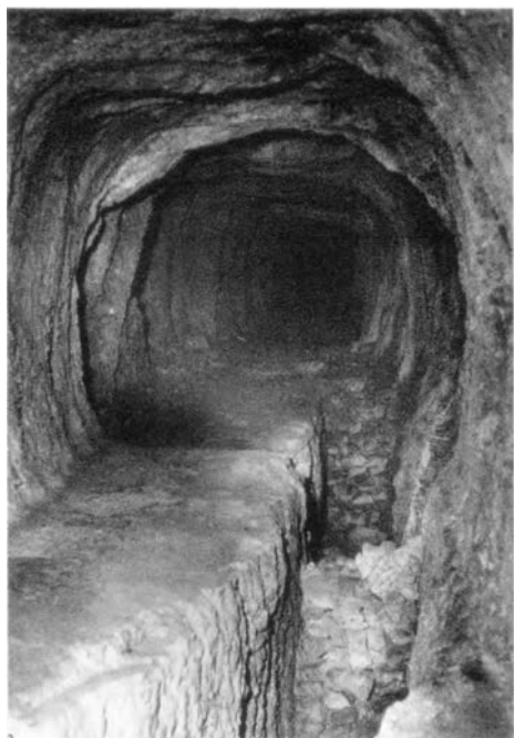
The tunnel of Eupalinos, piercing Mount Ampelus on Samos. It is mentioned by Herodotus as one of the three great achievements of Greek engineering (the other two, the Temple of Hera and the mole at what is now the harbor of Pythagorion, were also constructed on the island of Samos). Completed by the slaves of Polycrates, around 525 B.C.
