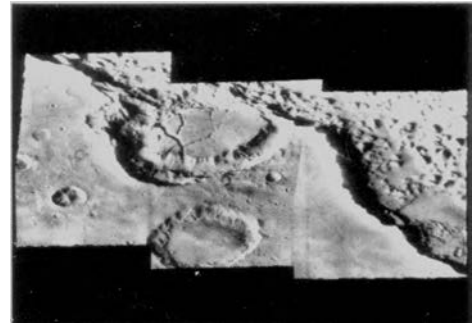
A crater on the northern escarpment of Capri Chasma, Mars. The slow enlargement of the valley has begun to crack and erode the crater. Mariner 9 photomosaic. Courtesy NASA.
