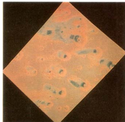
Windblown sand and dust in the lee of impact craters in Sinus Meridiani. Courtesy NASA.
