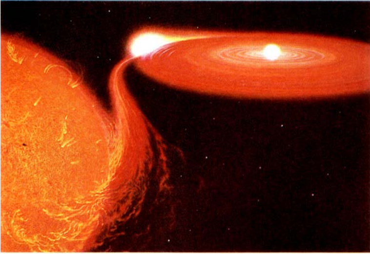
Late stages of stellar evolution. In a contact binary, the luminous stellar atmosphere flows from a red giant star ( left ) to the accretion disk around a pulsar neutron star ( right ). The disk glows in X-rays and other radiation at the point of contact. Painting by Don Davis.
