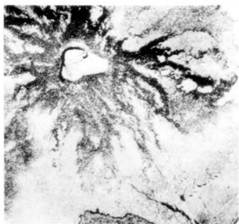
The Antarctic terrain of Io. A great profusion of landscapes can be seen ( top ), including smooth plains, volcanic calderas, sulfur flows, steep escarpments, and, at bottom right, surrounded by a bright halo, rugged and isolated mountains. The picture is about 1,700 kilometers across. At bottom is a close-up of a feature seen in the top picture at left center, a volcanic flow pattern 225 kilometers across, emanating from a caldera with an irregular island inside. Voyager 1 images. Courtesy NASA.
