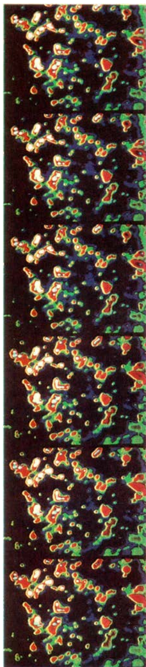
Atoms in motion: a motion picture film of disturbances in a carbon background (shown as blue-black) by the random motions of uranium atoms (shown as red). Democritus would have enjoyed this movie. Courtesy Albert Crewe, University of Chicago.
