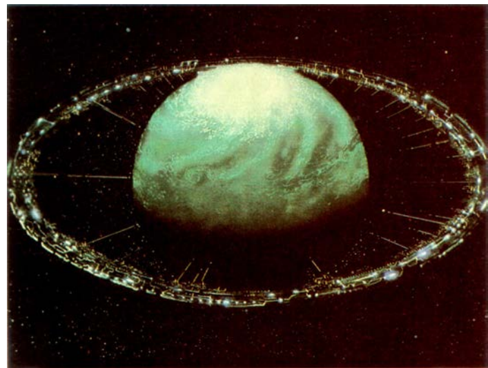
Hypothetical worlds from the Encyclopaedia Galactica . Top left and right: A planet and its two moons, their surfaces destroyed by a nearby supernova explosion. Middle left and right: An oceanic Earth-like world with two large moons. Lower left: A terrestrial planet with major engineering work visible on its night side. Somewhat more advanced than we, it is a candidate transmitting civilization for our first interstellar radio message. Lower right: A still more advanced civilization, constructing a habitable ring system about its home planet. Paintings, respectively, by Rick Sternbach, David Egge, Rick Sternbach, David Egge, John Allison and Jon Lomberg.
