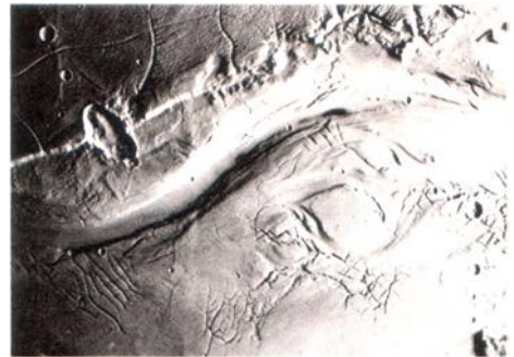
A portion of Kasei Vallis, an ancient river valley on Mars. Kasei is Japanese for Mars. The impact craters in the channel floor are evidence of its great age. Abundant surface liquid water earlier in Martian history suggests that conditions for life were once more favorable. Viking Orbiter photo, courtesy NASA.
