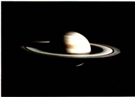
Saturn. Model by Adolf Schaller, Rick Sternbach and John Allison.
