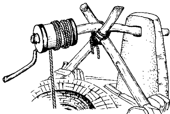
辘 轳
